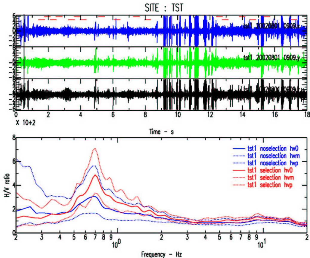
Fig. 5. Signal (top) processed with (red curves bottom) or without (blue curves bottom) the automatic window selection (selected windows are indicated by the red segments on the top of the signal). The peak on the H/V curve is much clearer when the transient removal is applied, and also the standard deviation is lower, especially at low frequencies.
