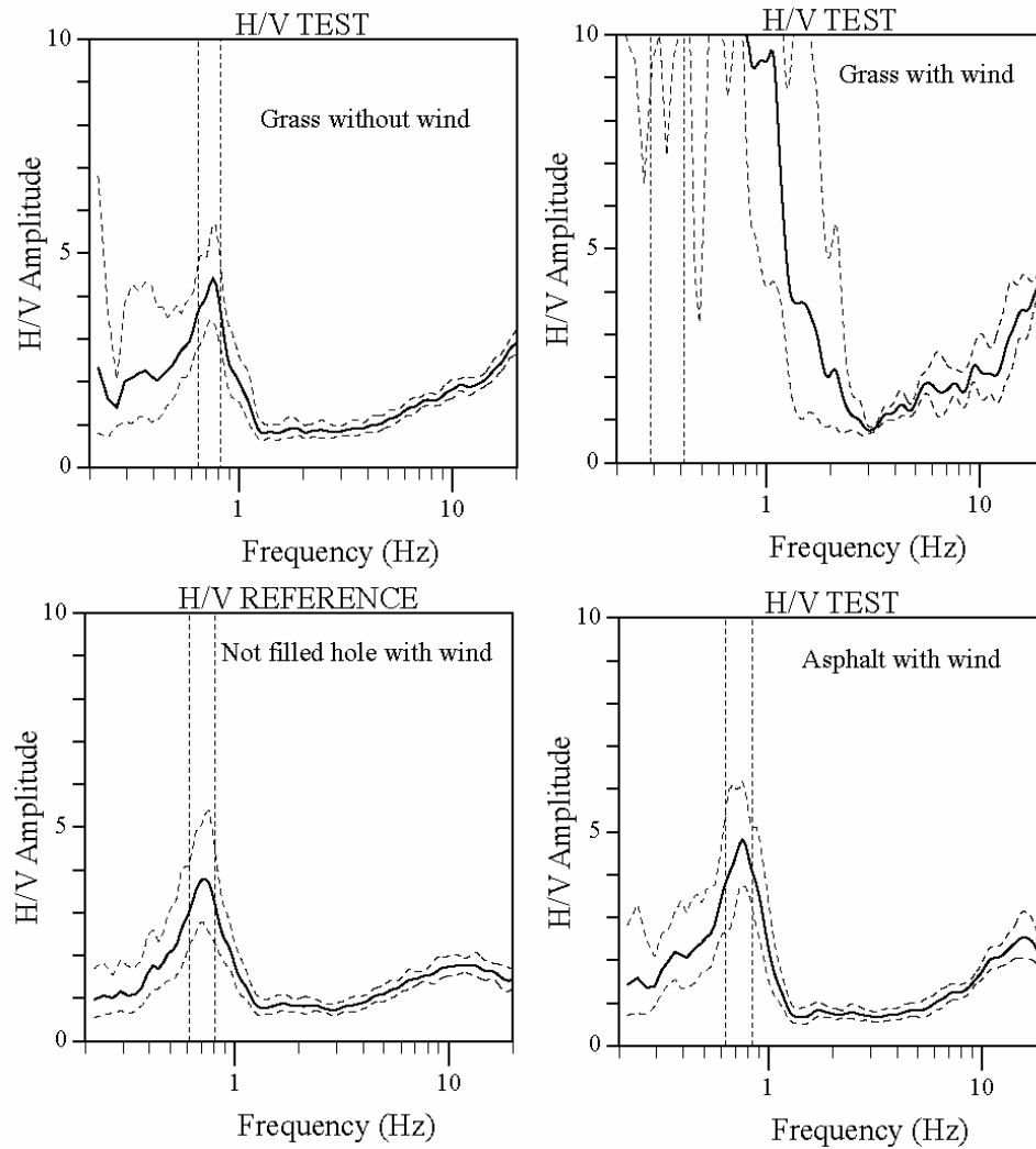
Fig. 2. Comparison of the H/V curves obtained at the same site on grass with and without wind (top), and in a hole, on asphalt (bottom) and again on grass with wind. This comparison shows the strong effect of the wind combined with grass, whereas on asphalt or in a hole, the wind has no significant effect (if far away from any structure).
