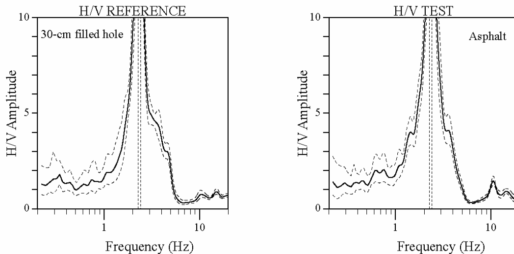
Fig. 1. Comparison of the H/V curves obtained with and without asphalt, at the same site, showing no significant effect of the asphalt layer.
