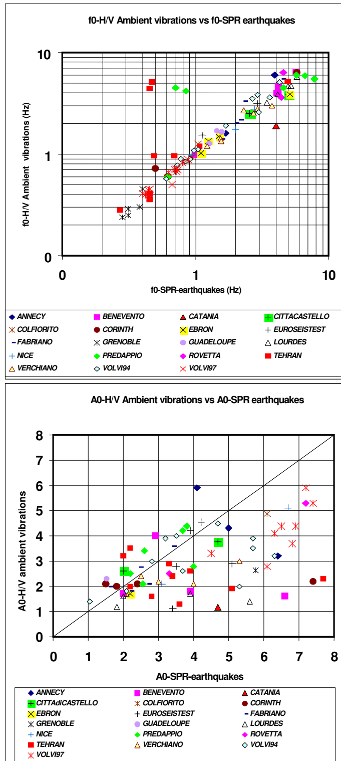
Fig. 8. Comparison between H/V ratio of ambient vibrations and standard spectral ratio of earthquakes. Top: comparison of the frequencies f_0 , bottom: comparison of the amplitudes A_0 .
