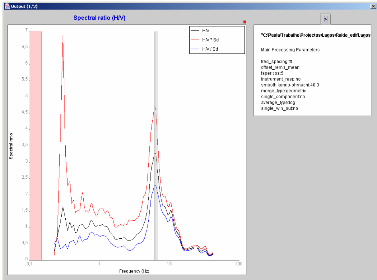
Fig. 6. H/V ratio for the merged horizontal components (mean in black, mean multiplied and divided by 10^{\sigma(\log H/V)} , in red and blue). The pink strip shows the frequency range where the data has no significance, due to the sampling rate and the window length. The grey strip represents the mean f_0 , plus and minus the standard deviation. It is calculated from the f_0 of each individual window.
