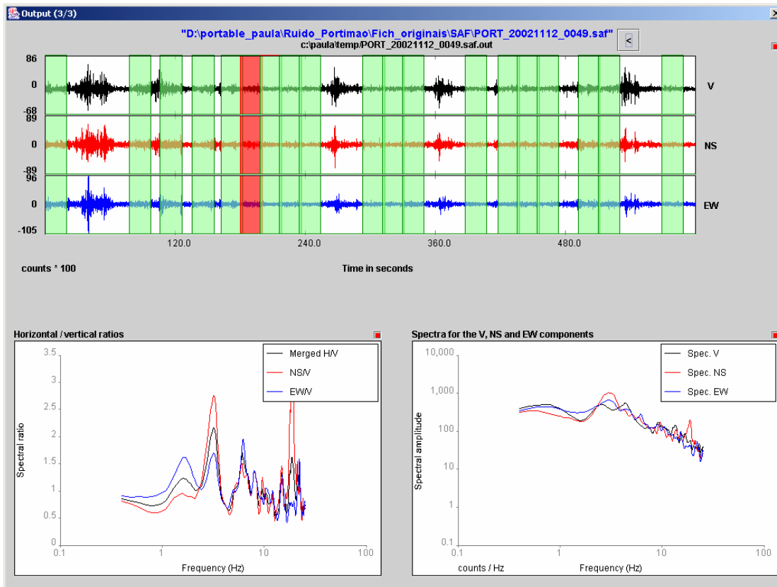
Fig. 7. Result for individual windows: H/V ratios and spectra shown are derived from the signal displayed in the red window.
