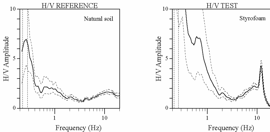
Fig. 3. Comparison of the H/V curves obtained with and without a Styrofoam plate under the sensor, at the same site, showing a strong effect of the Styrofoam.
